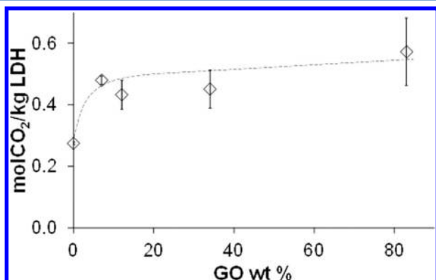
Figure 7. Average CO 2 sorption capacities per mass of LDH at 573 K and P(\text{CO}_2) = 0.2 bar, based on measured GO content, shown with standard errors.
