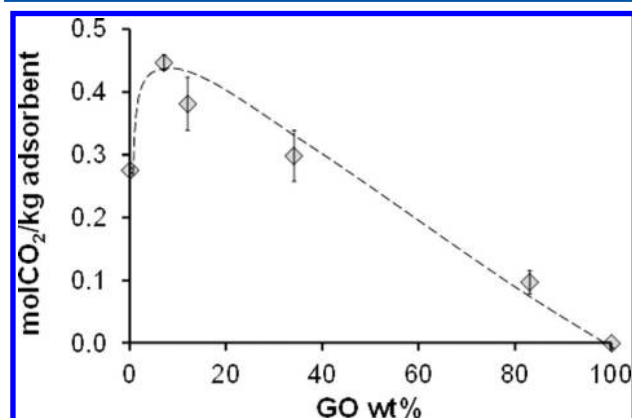
Figure 8. Average CO 2 sorption capacities per mass of total adsorbent of pure LDH and carbon hybrids at 573 K and P(\text{CO}_2) = 0.2 bar, based on measured GO content, shown with standard errors.
