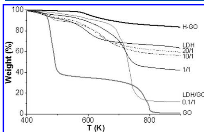
Figure 2. Thermograms of unsupported LDH and LDH/GO hybrid samples. The nominal loading is indicated in the figure, and the deduced actual loading data are in Table 1. Repeated sample traces indicated negligible error.
